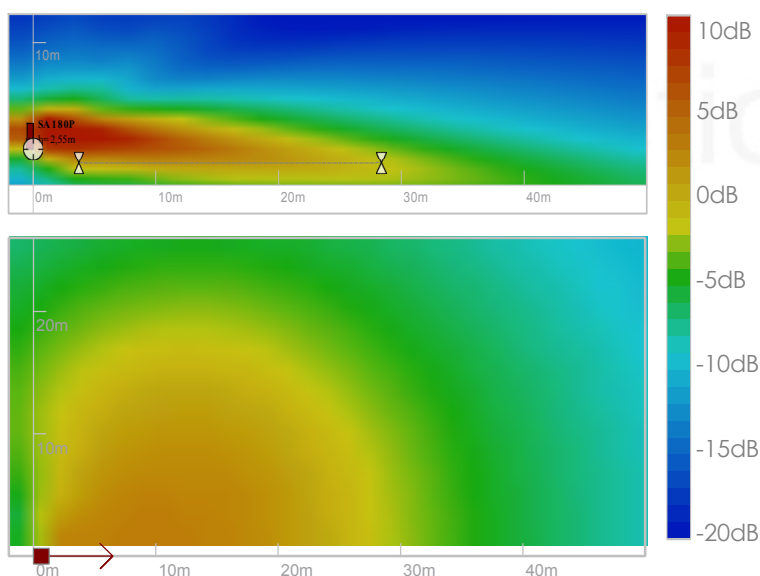
Abscissa: distance (m). Column SA180P at 2,55m from ground. 0 dB is the mean SPL over 6m-25m on axis.
