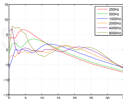
Abscissa: distance (m). Column SA180P at 2,55m from ground. 0 dB is the mean SPL over 6m-25m on axis.
